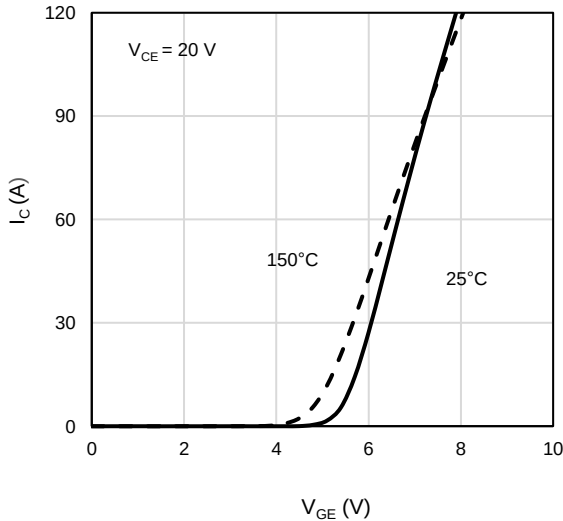
Figure 6: Transfer Characteristics
