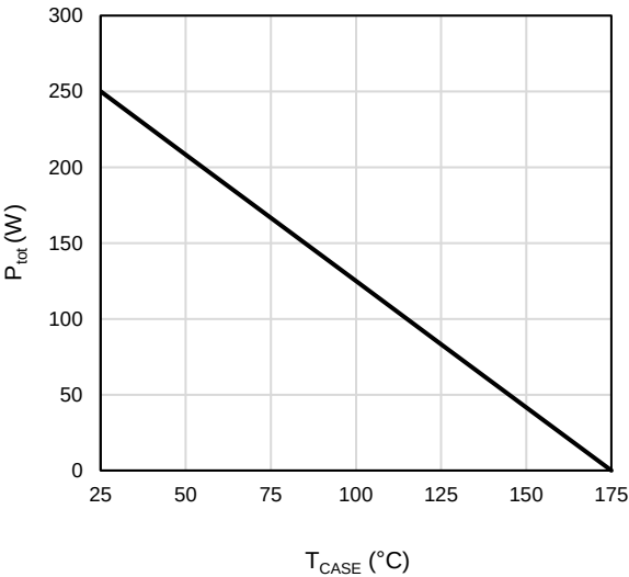
Figure 1: Power De-rating
